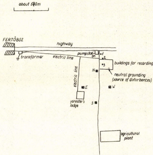
Fig. 2. General plan of the Nagyccenk Observatory
