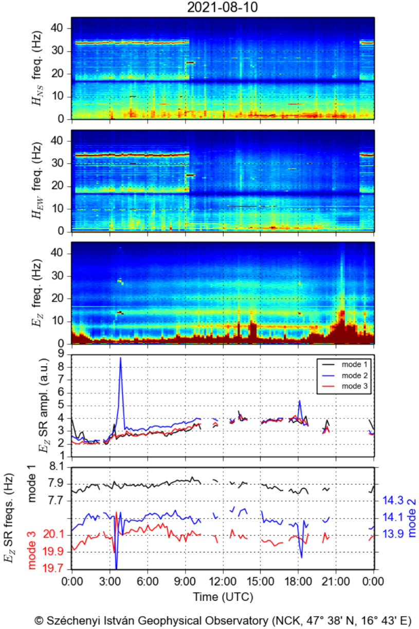
Fig. 2: The automatically generated figure showing the Schumann resonance measurements at the SZIGO on the 10 th of August, 2021.
