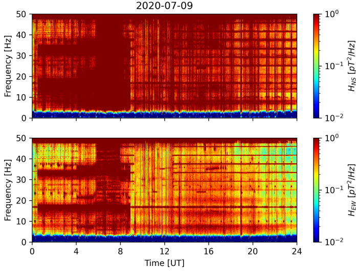
Fig. 1: Dynamic spectra corresponding to the H_{NS} (top panel) and H_{EW} (bottom panel) field components from the day of the noise test which began at 08:45 UT and ended at 11:30 UT.
